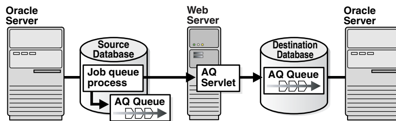
Figure 6-2 HTTP Oracle Streams Advanced Queuing Propagation
