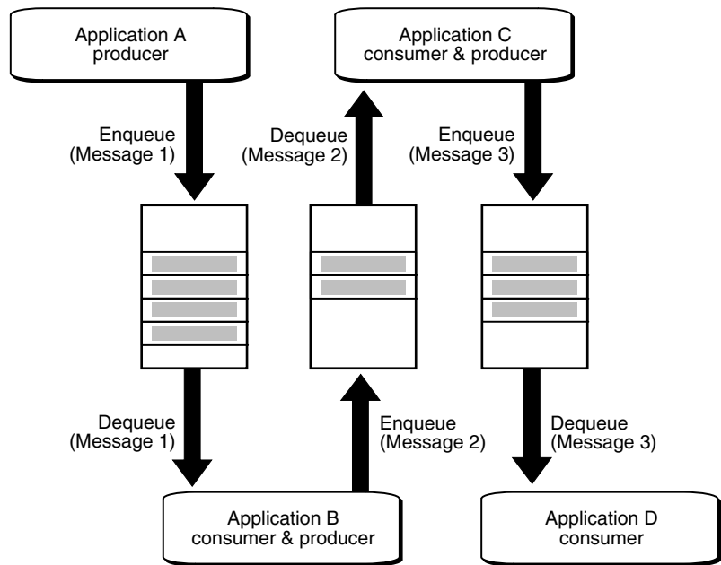
Figure 1-5 Implementing a Workflow using Oracle Streams Advanced Queuing
