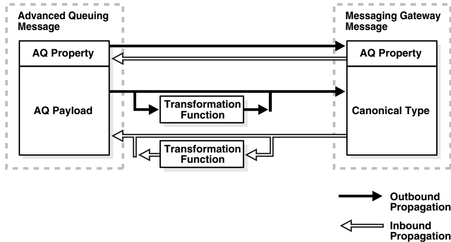
Figure 20–2 Oracle Streams Advanced Queuing Message Conversion
