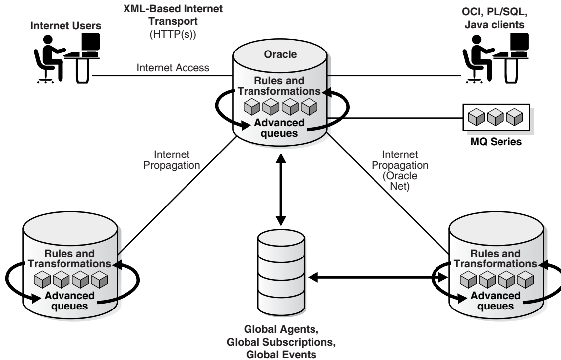
Figure 1-1 Integrated Application Environment Using Oracle Streams Advanced Queuing
