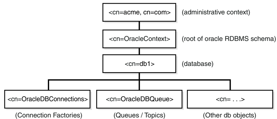
Figure 11-1 Structure of Oracle Streams Advanced Queuing Entries in LDAP Server
