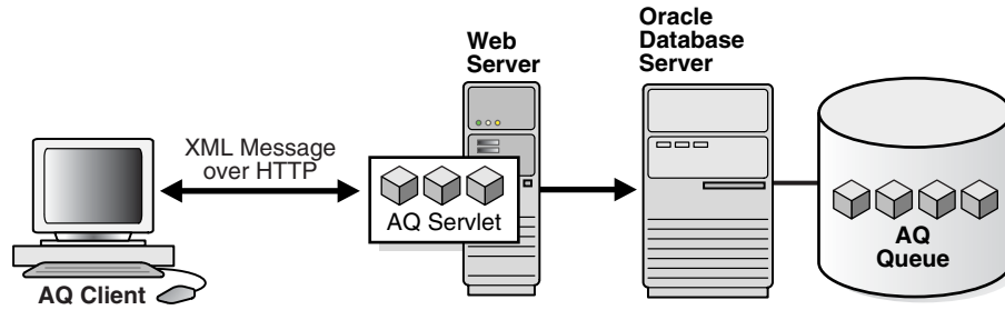
Figure 1–11 Architecture for Performing Oracle Streams Advanced Queuing Operations Using HTTP
