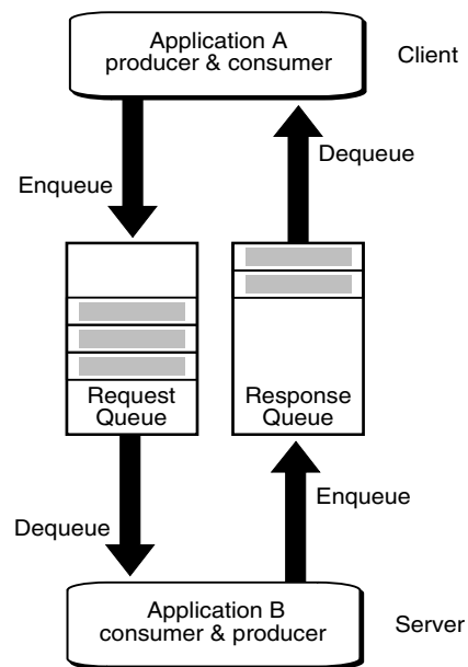
Figure 1–2 Client/Server Communication Using Oracle Streams Advanced Queuing
