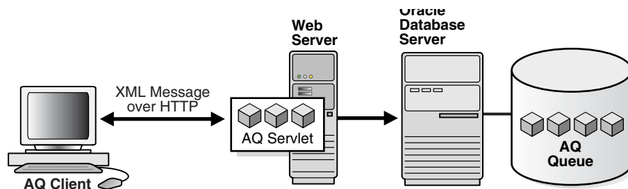
Figure 6–1 Architecture for Performing Oracle Streams Advanced Queuing Operations Using HTTP
