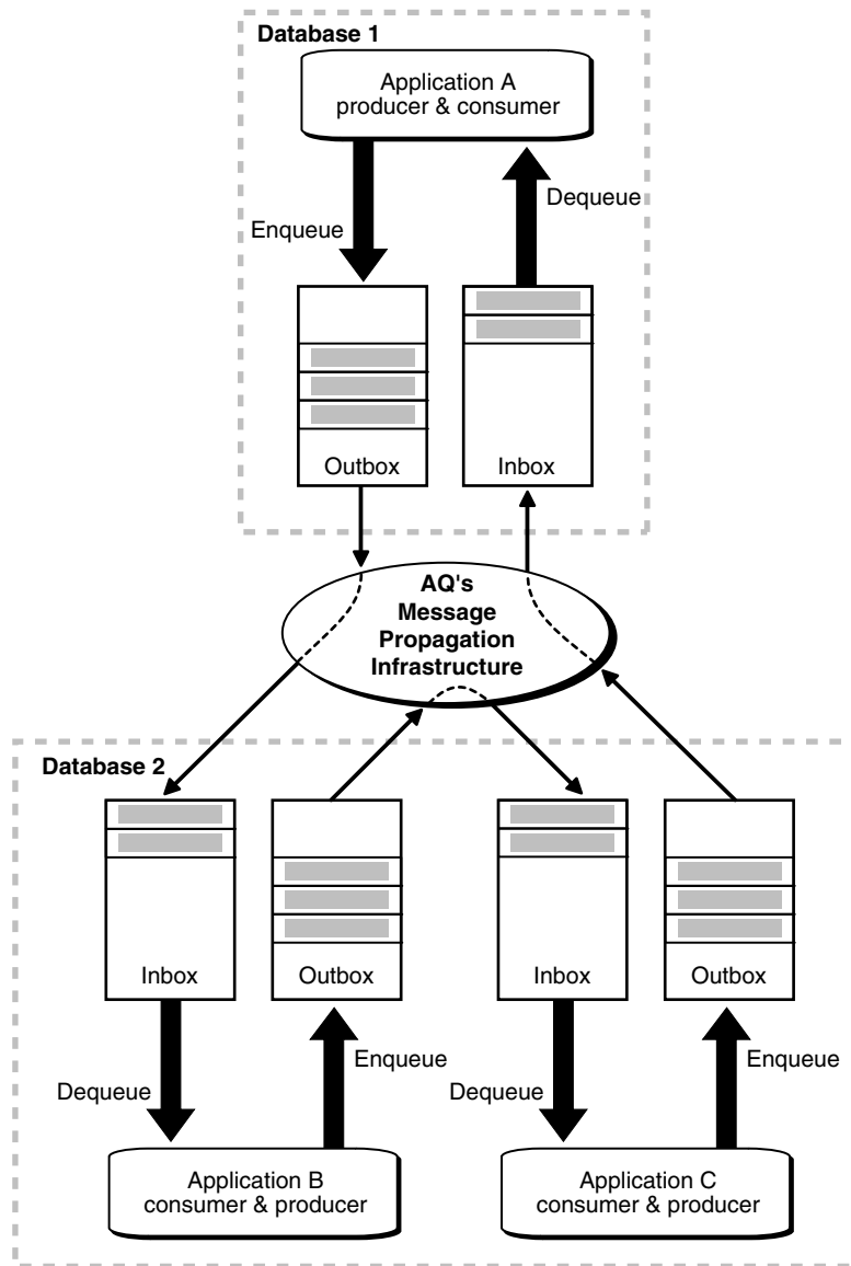
Figure 1–9 Message Propagation in Oracle Streams Advanced Queuing
