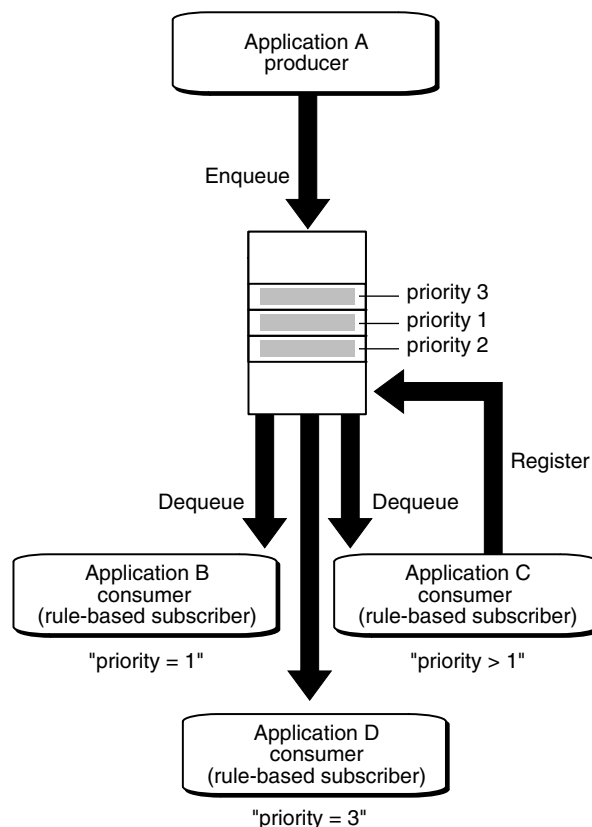
Figure 1–8 Implementing Publish/Subscribe using Oracle Streams Advanced Queuing
