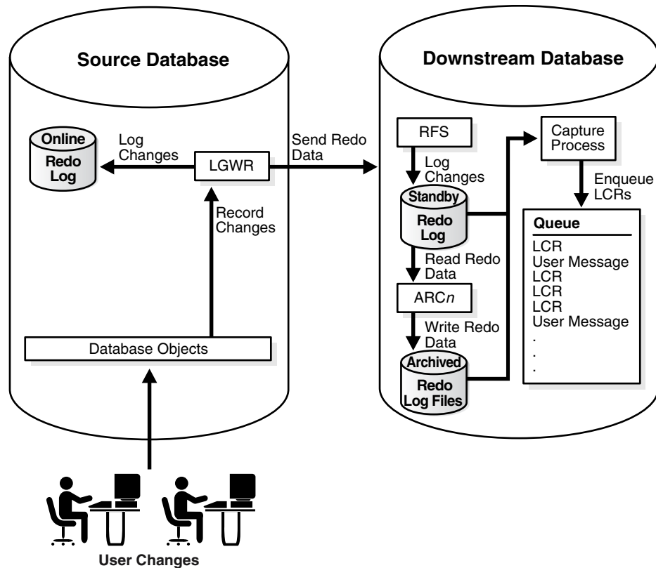
Figure 2–2 Real-Time Downstream Capture
