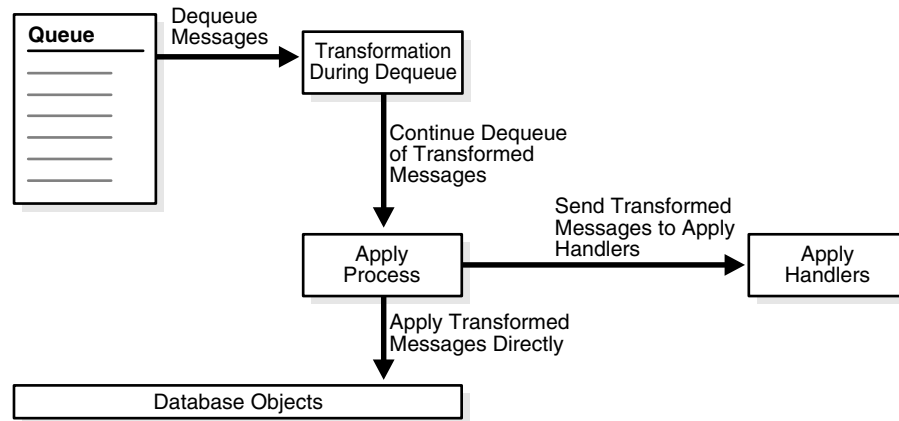
Figure 6–4 Transformation During Apply
