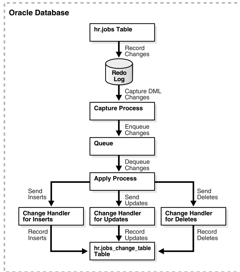
Figure 20–1 Recording Changes Using Local Capture and Apply on One Database
