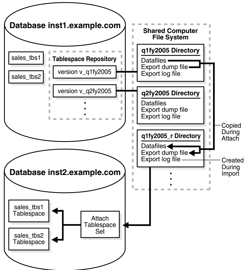
Figure 36–2 Attaching Tablespaces with a Shared File System
