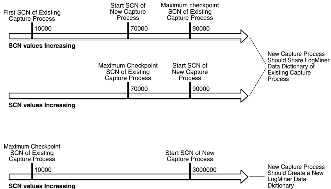
Figure 7–4 Deciding Whether to Share a LogMiner Data Dictionary
