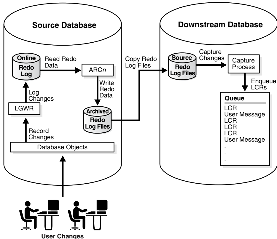
Figure 2-3 Archived-Log Downstream Capture
