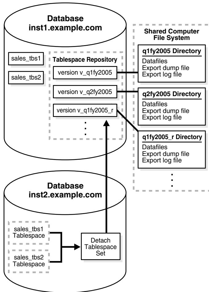
Figure 36-3 Detaching Tablespaces with a Shared File System
