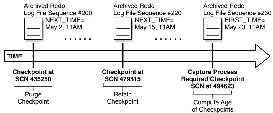
Figure 7–1 Checkpoint Retention Time Set to 20 Days
