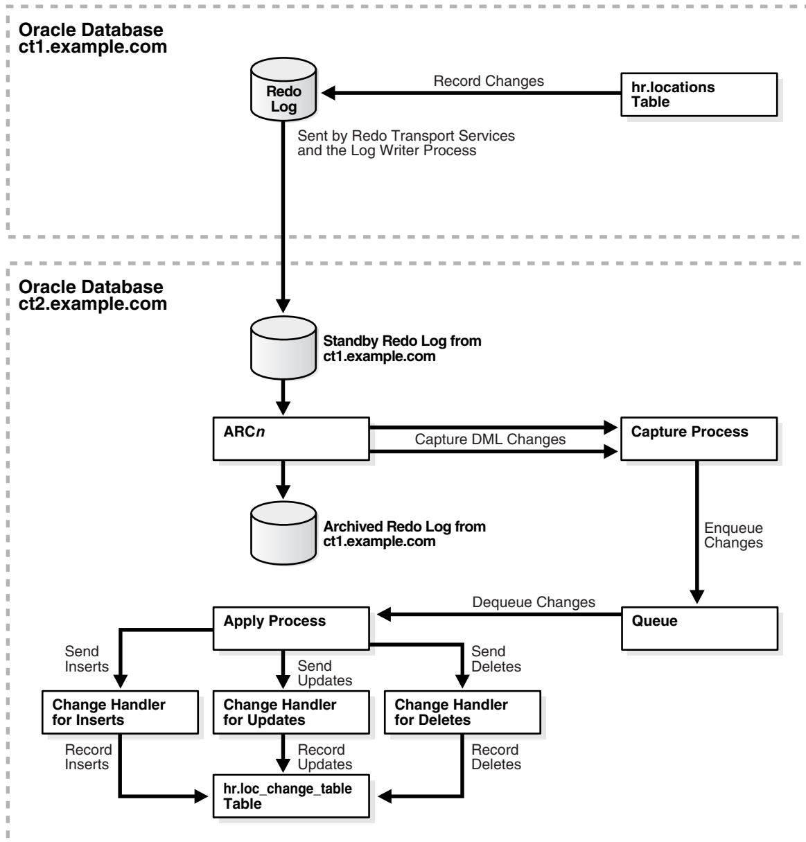
Figure 20-3 Recording Changes Using Downstream Capture and Local Apply
