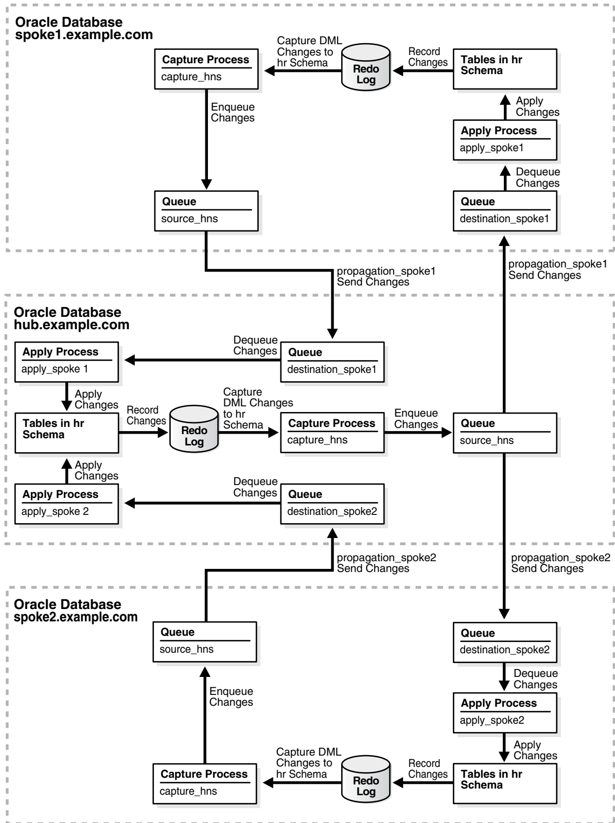
Figure 23–3 Sample Oracle Streams Replication Environment
