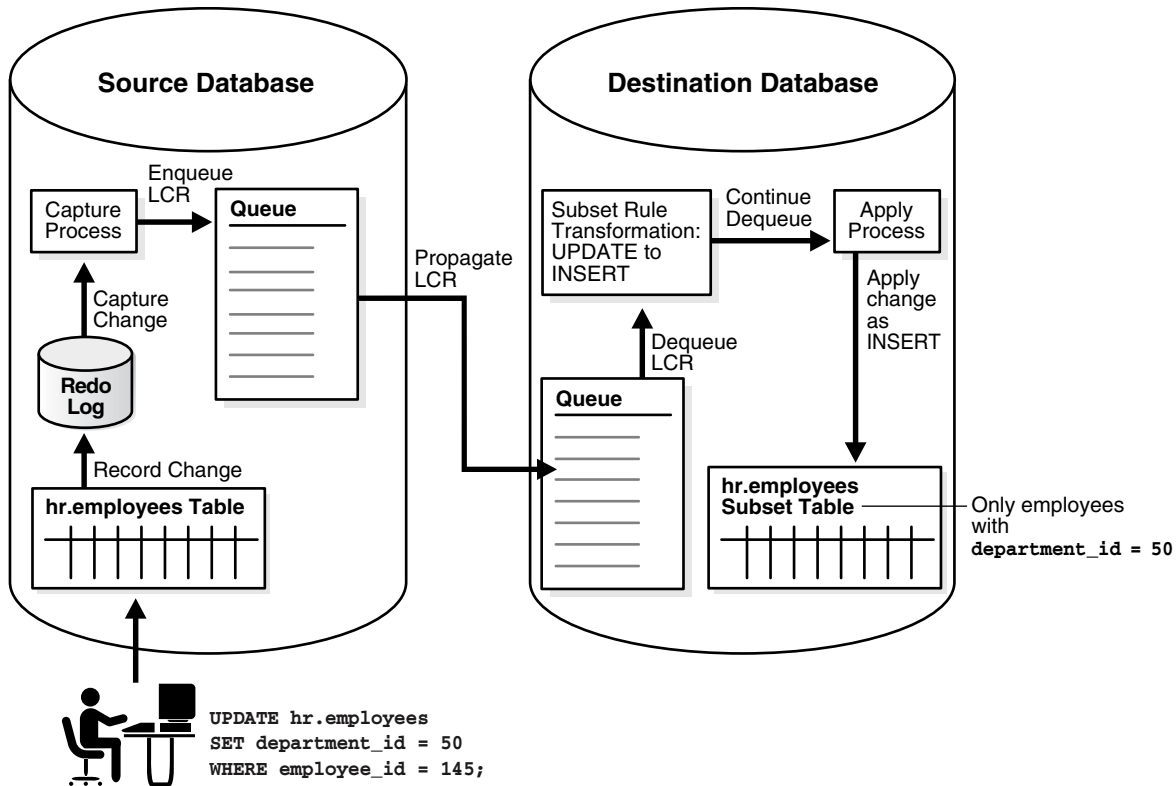
Figure 5–4 Row Migration During Apply
