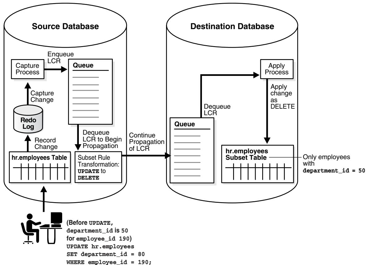
Figure 5-3 Row Migration During Propagation
