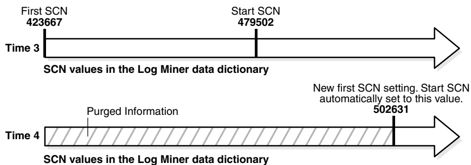
Figure 7-3 Start SCN Lower than Reset First SCN
