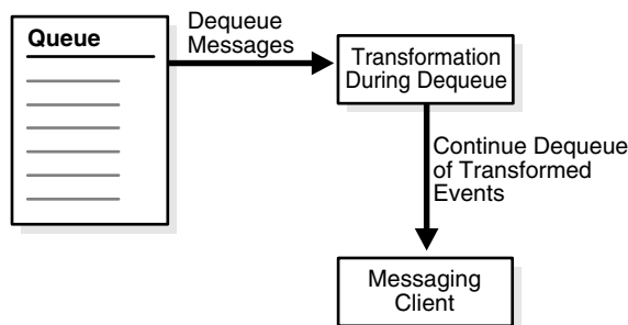
Figure 6–5 Transformation During Messaging Client Dequeue
