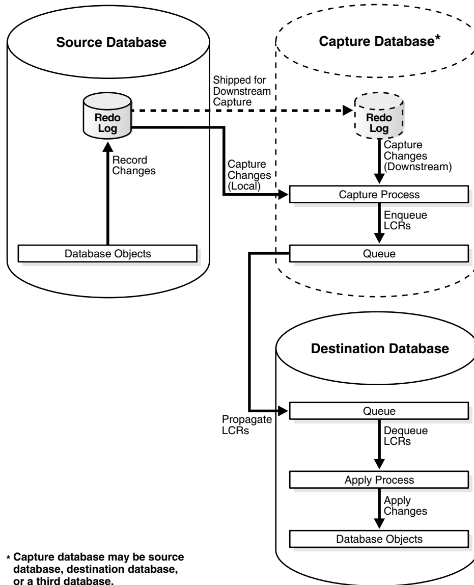
Figure E-1 Online Database Upgrade with Oracle Streams
