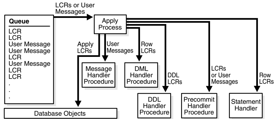
Figure 4–1 Apply Process Message Processing Options
