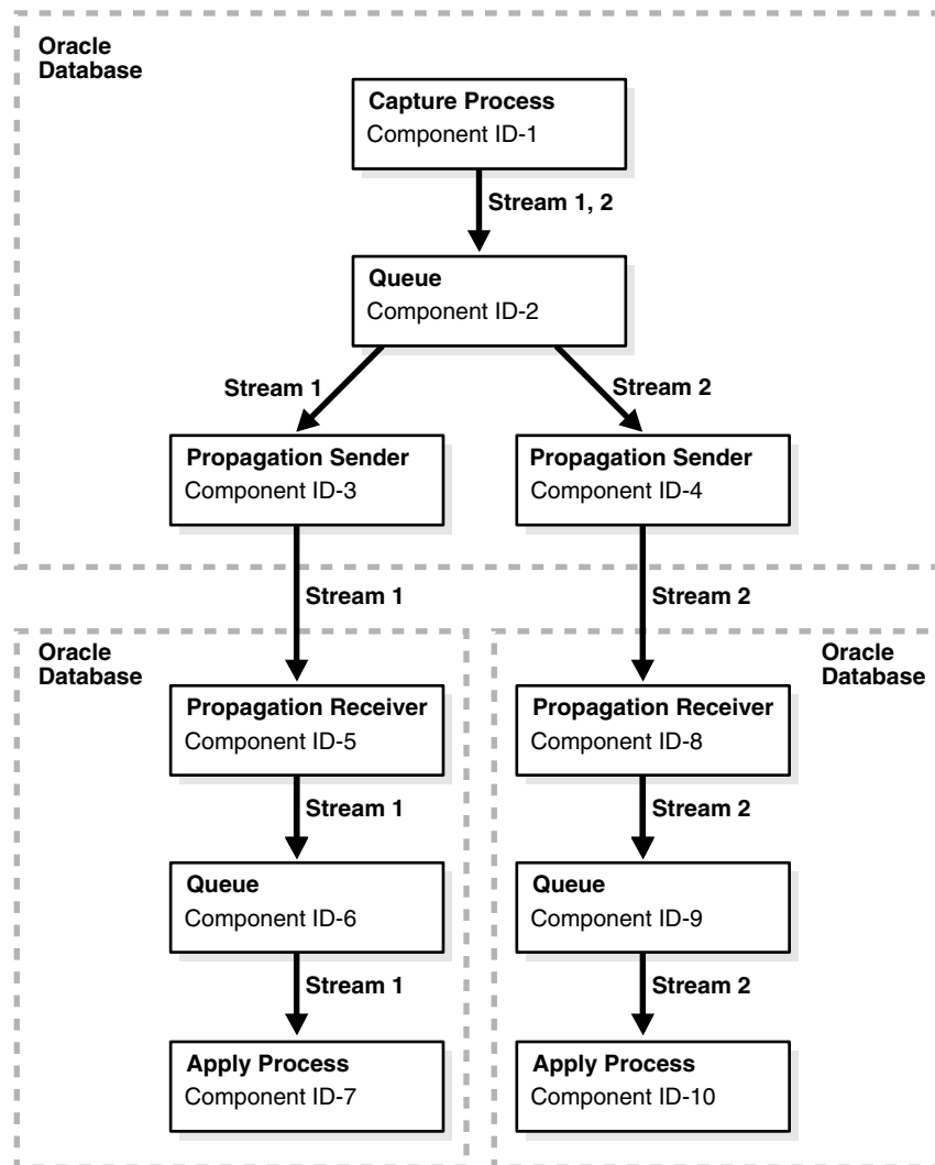
Figure 23–2 Oracle Streams Topology with Multiple Apply Processes for a Single Source
