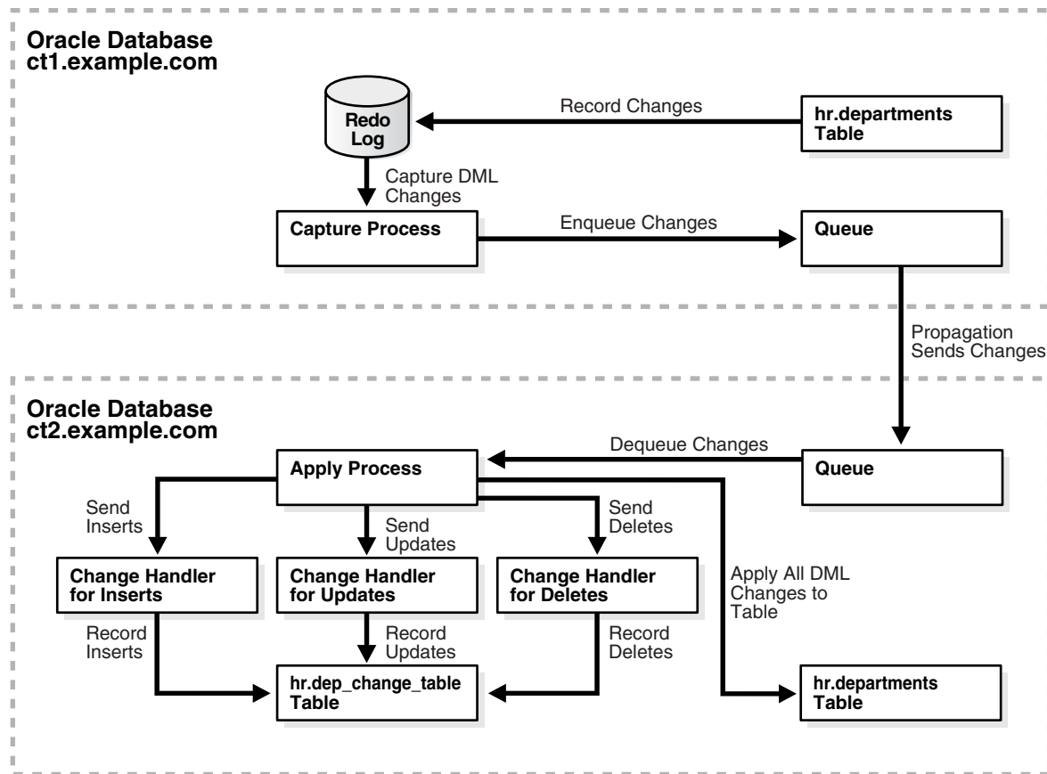
Figure 20–2 Recording Changes Using Local Capture and Remote Apply with Replication
