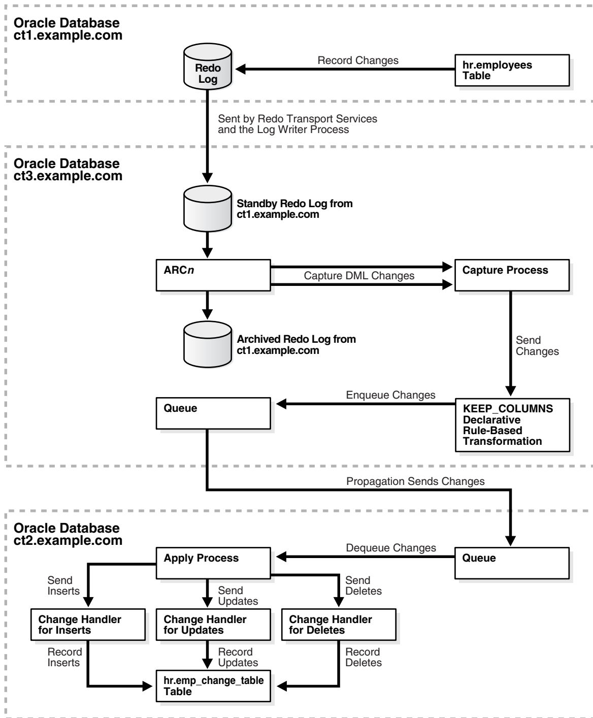
Figure 20-4 Recording Changes Using Downstream Capture and Remote Apply
