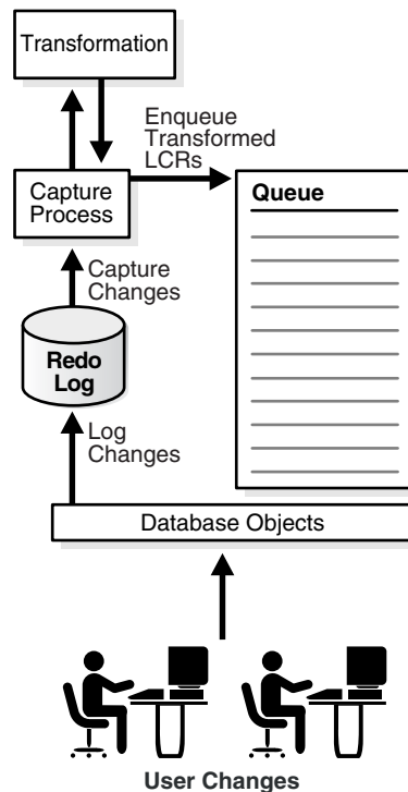
Figure 6-1 Transformation During Capture by a Capture Process
