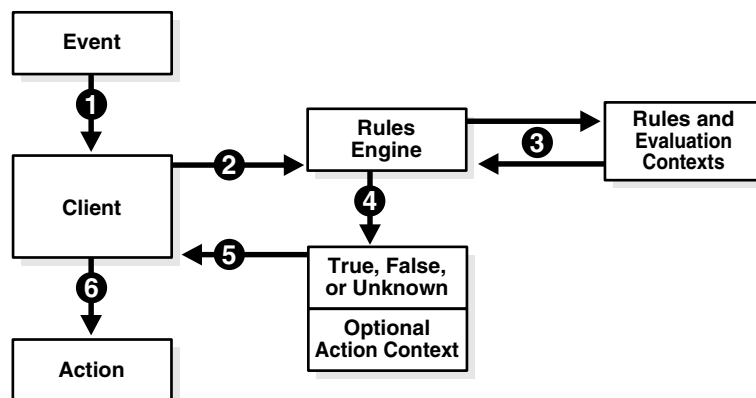
Figure 11–1 Rule Set Evaluation
