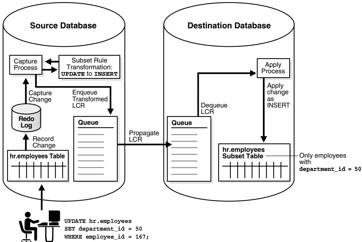
Figure 5–2 Row Migration During Capture by a Capture Process
