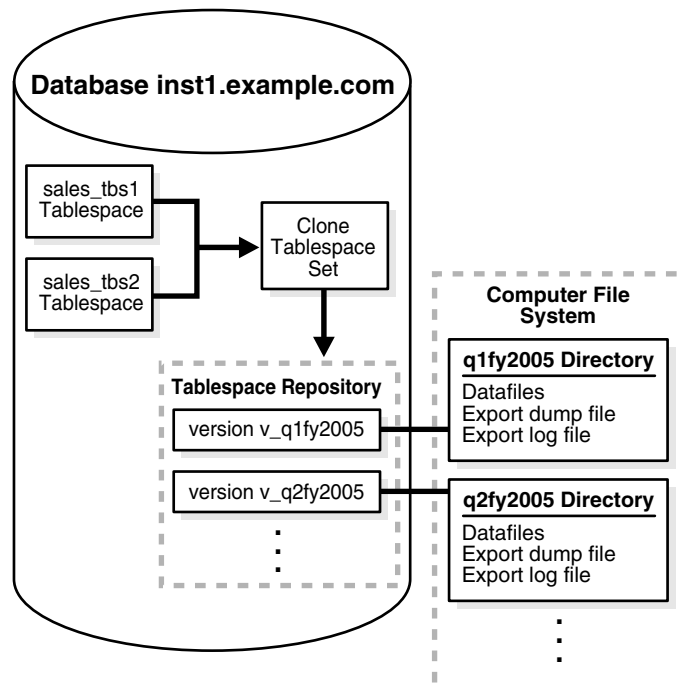
Figure 36–1 Example Tablespace Repository
