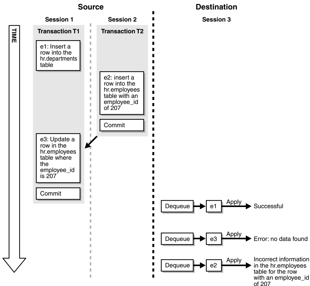
Figure 8–1 Transactional Dependency Violation During Dequeue
