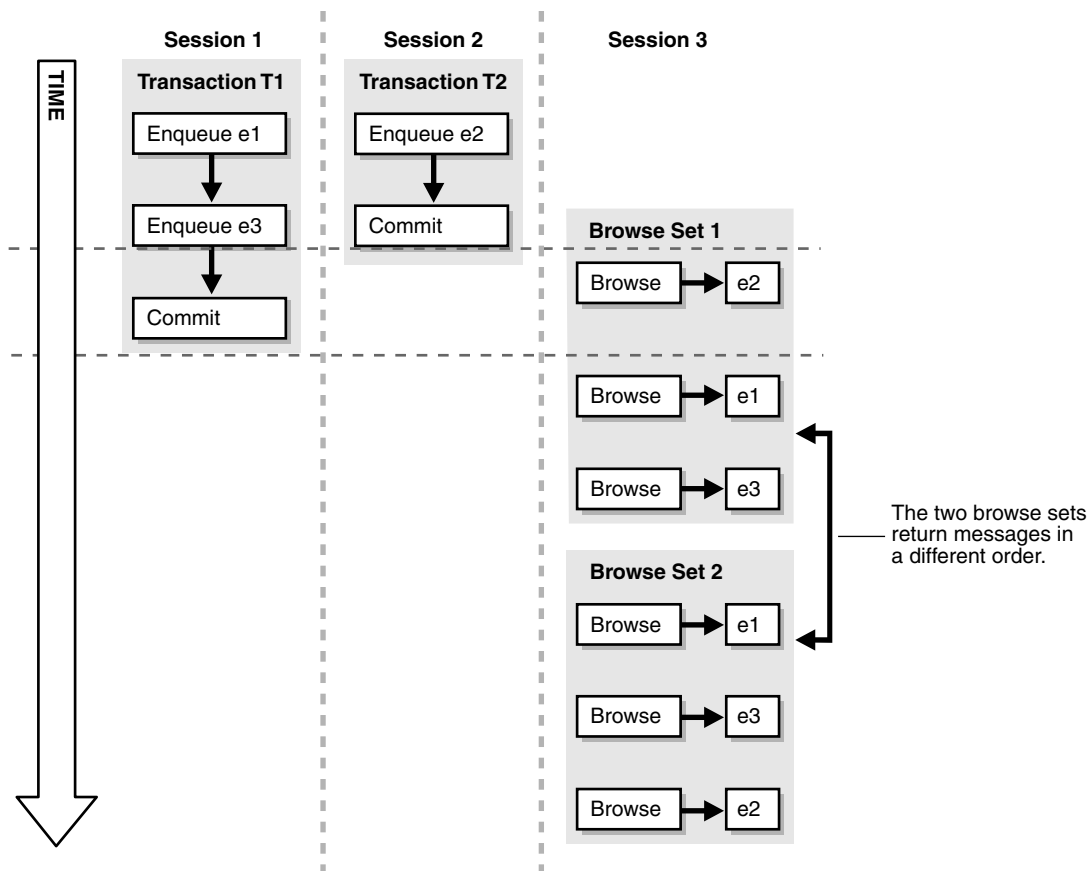
Figure 8–2 Inconsistent Browse of Messages in a Queue
