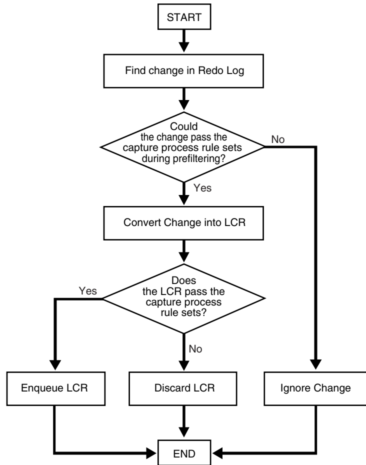
Figure 7-5 Flowchart Showing Capture Process Rule Evaluation
