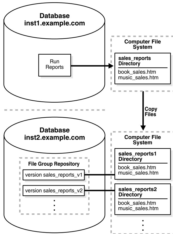
Figure 36-5 Example File Group Repository
