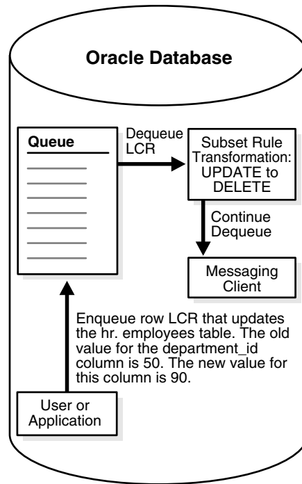
Figure 5–5 Row Migration During Dequeue by a Messaging Client
