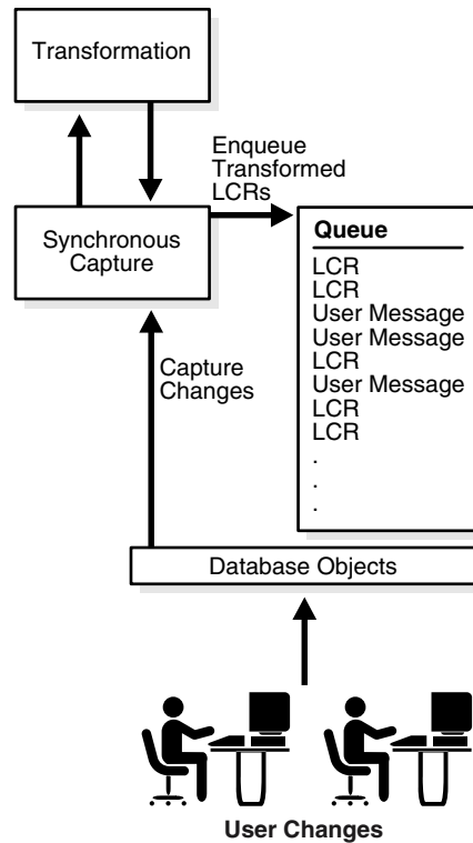
Figure 6–2 Transformation During Capture by a Synchronous Capture
