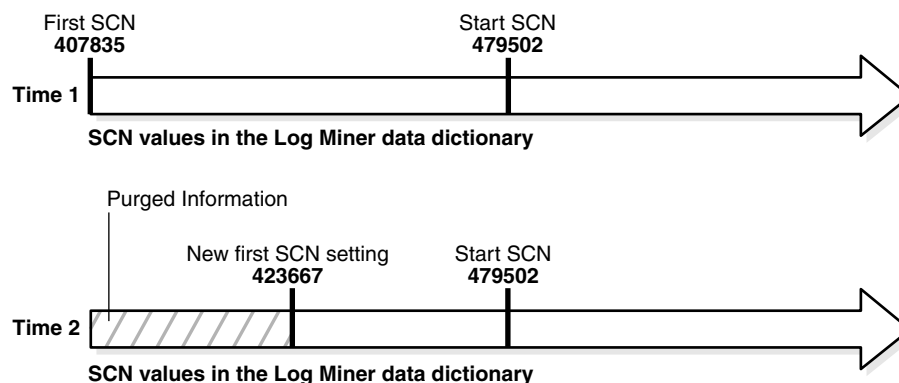
Figure 7-2 Start SCN Higher than Reset First SCN
