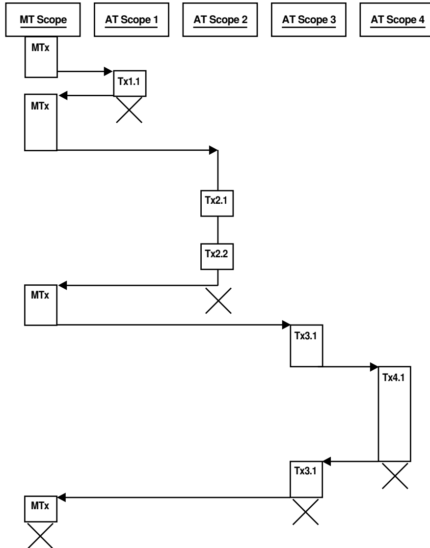
Figure 8-4 Possible Sequences of Autonomous Transactions
