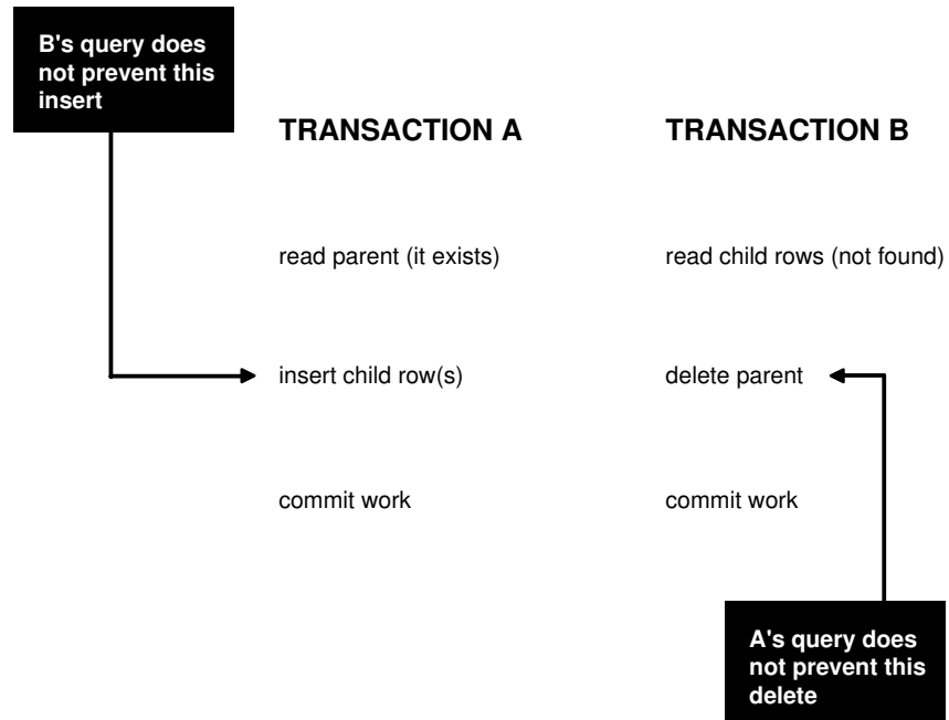
Figure 8-2 Referential Integrity Check
