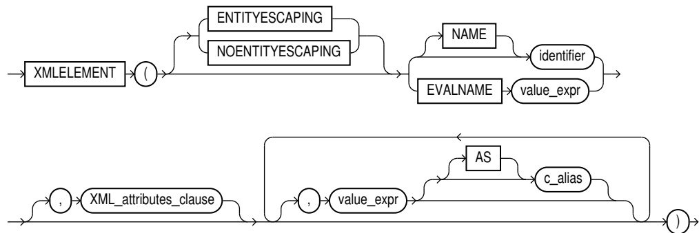
Figure 8-1 XMLELEMENT Syntax
