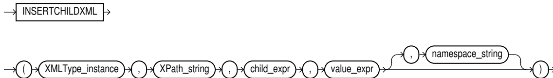
Figure C-2 INSERTCHILDXML Syntax
