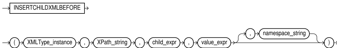
Figure C-3 INSERTCHILDXMLBEFORE Syntax
