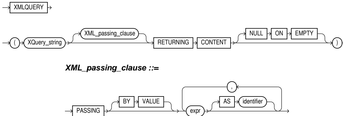
Figure 4-1 XMLQUERY Syntax
