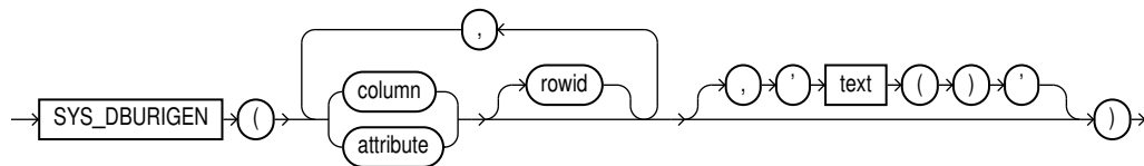
Figure 32-2 SYS_DBURIGEN Syntax
