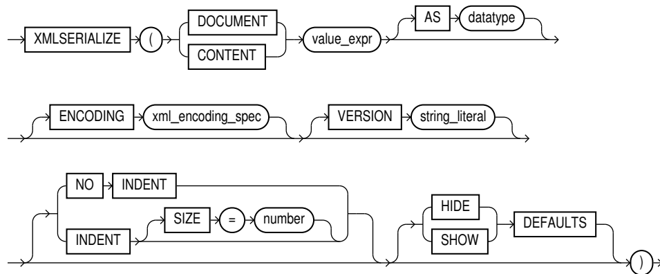
Figure 8-8 XMLSerialize Syntax
