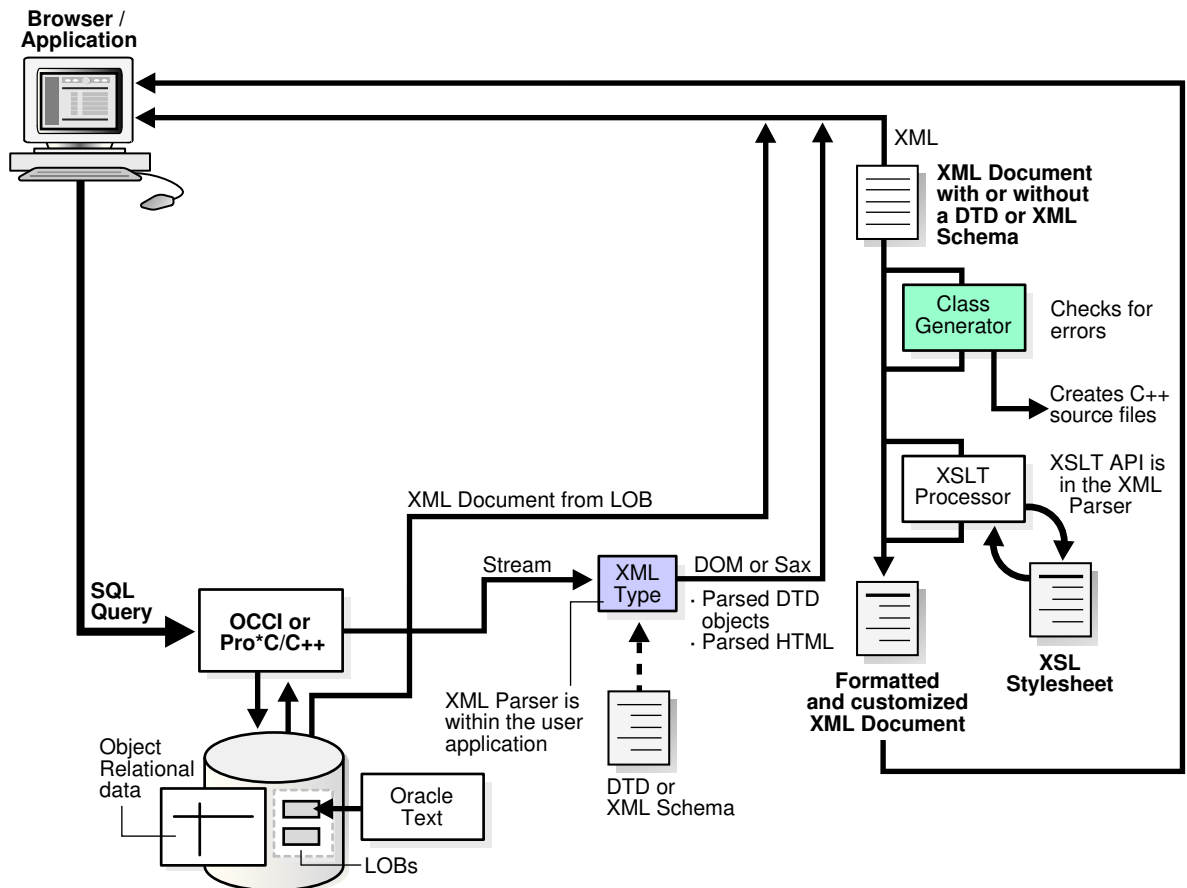
Figure 1-9 Generating XML Documents Using Oracle XML Developer's Kit C++ Components
