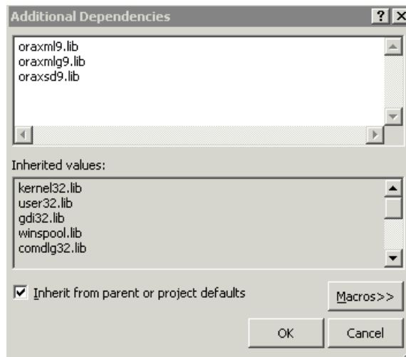
Figure 18-4 Setting the Names of the Libraries in Visual C++ Project
