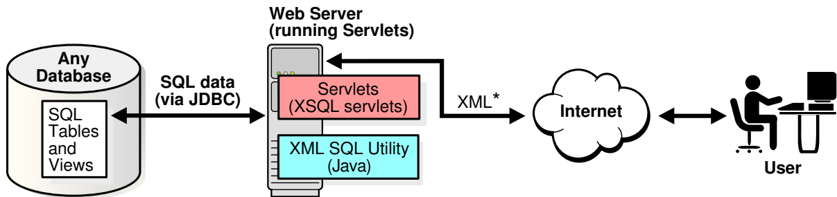
Figure 13-5 Running XSU in a Web Server
