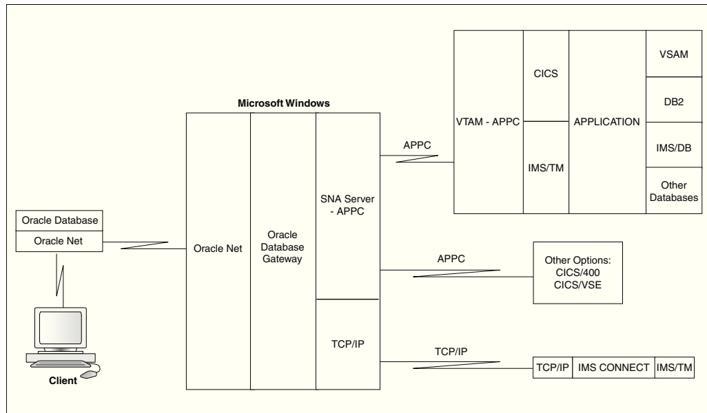
Figure 1-2 Gateway Architecture
