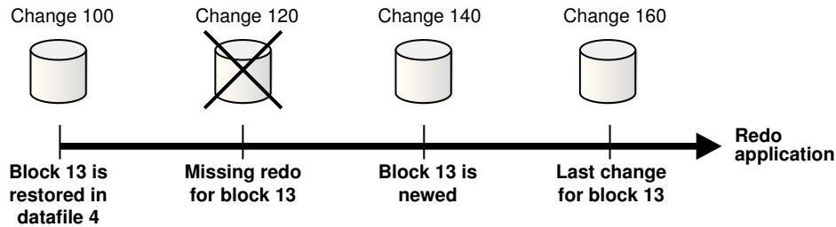
Figure 19-1 Performing RMAN Media Recovery
