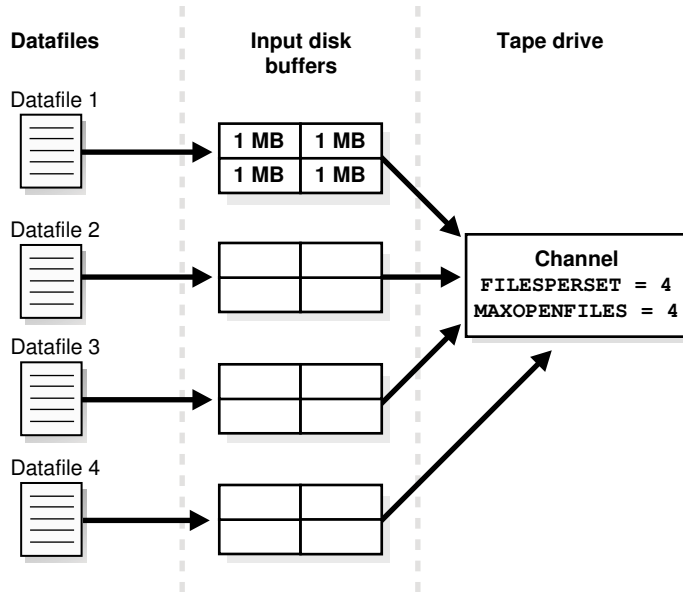
Figure 23-3 Disk Buffer Allocation
