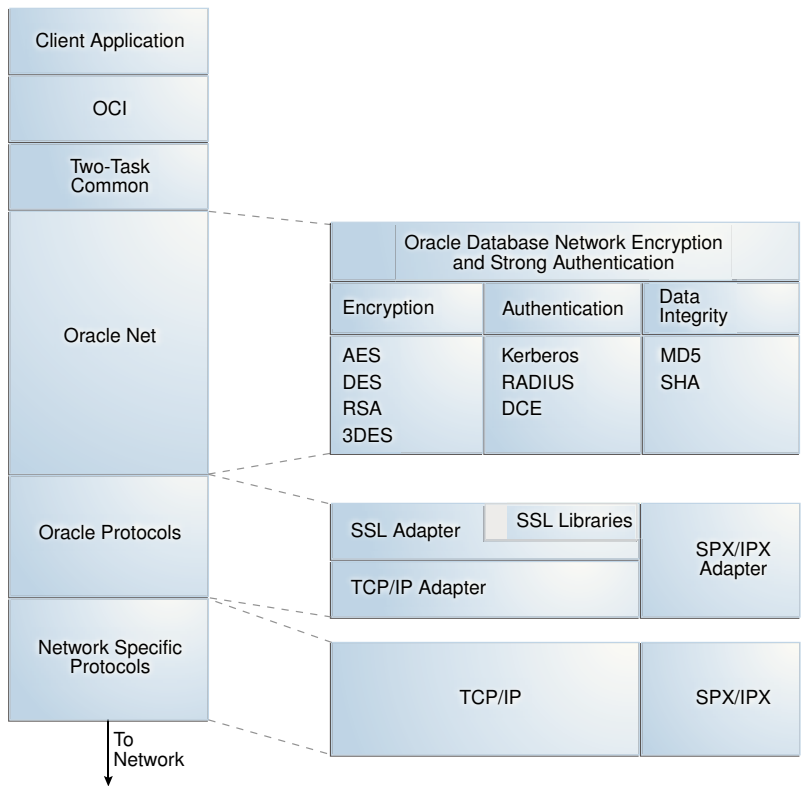
Figure 15-3 Oracle Network Encryption and Strong Authentication Architecture
