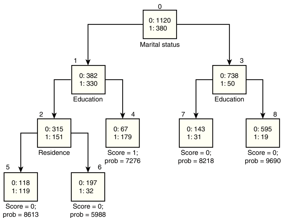
Figure 10-2 Sample Decision Tree
