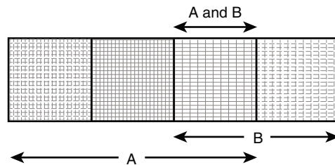
Figure 17-1 Conditional Probabilities in Bayes' Theorem
