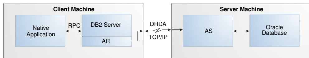
Figure 1-2 Native Application Remote Connectivity Model
