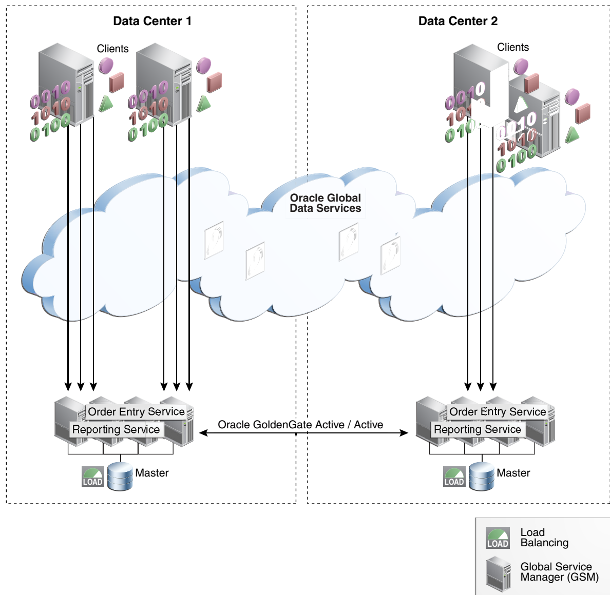
Figure 1-6 Region Affinity in Oracle GoldenGate Multi-Master
