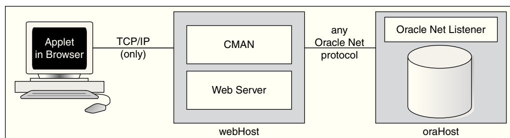
Figure 5-1 Applet, Connection Manager, and Database Relationship
