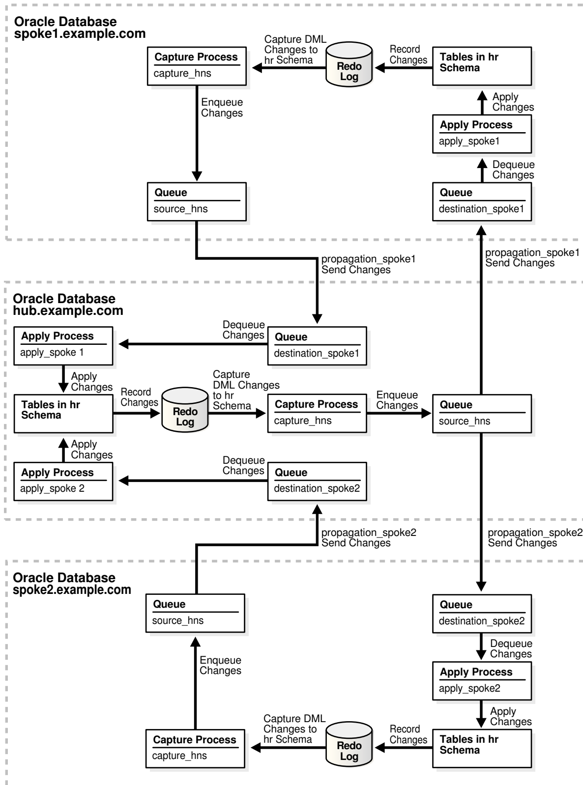
Figure 23-3 Sample Oracle Streams Replication Environment
