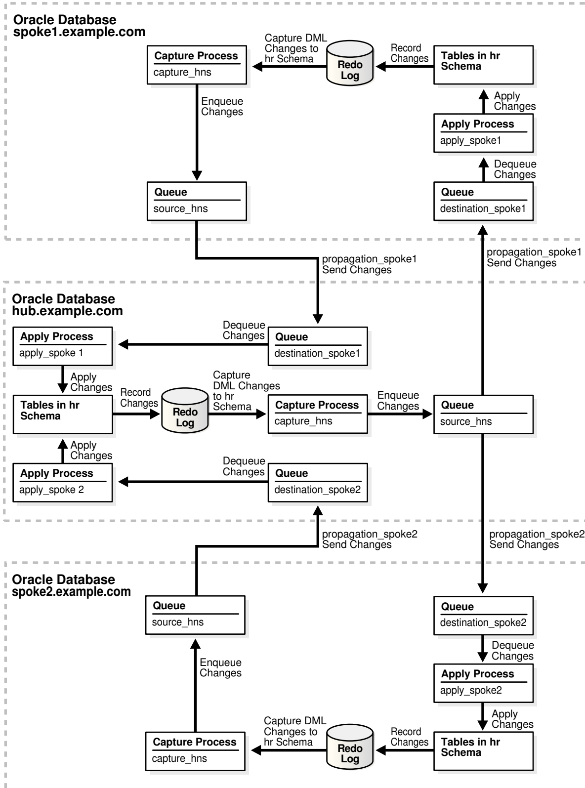
Figure 1-2 Sample Hub-and-Spoke Replication Configuration
