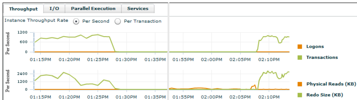
Figure 4-10 Monitoring Throughput
