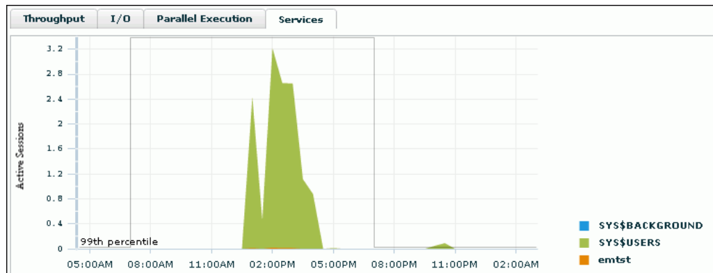
Figure 4-13 Monitoring Services
