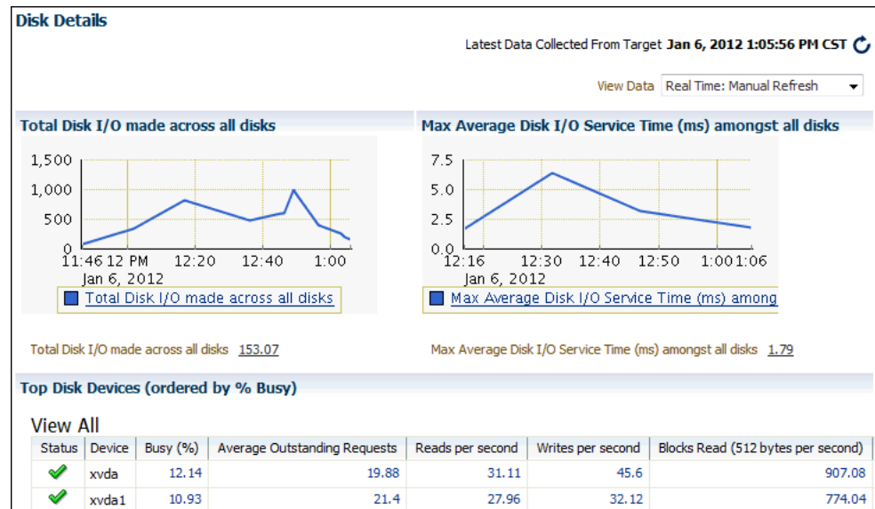
Figure 4-16 Disk Details
